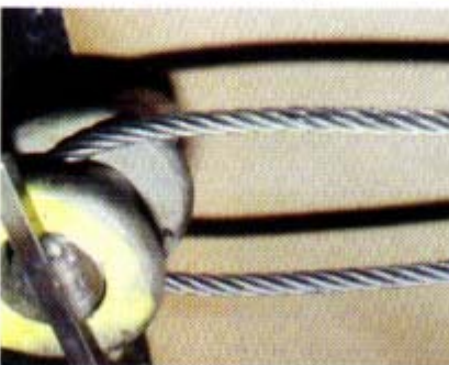
Photo #5 Wire rope pin test - 4/1 D/d ratio
