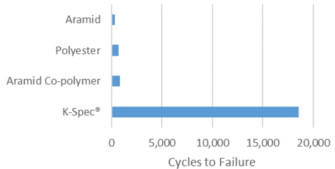
Figure 1- Yarn on Yarn Abrasion Results
